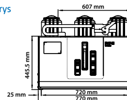
Bokorys
